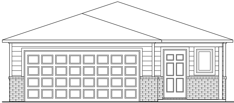
RC Tucson Elevation A
