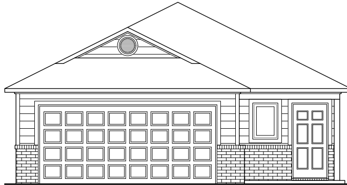
RC Mitchell Elevation I
