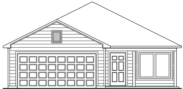
RC Carlisle Elevation J
