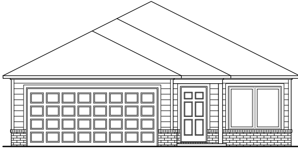
RC Carlisle Elevation A
