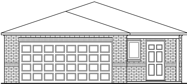
RC Tucson Elevation C
