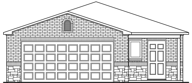
RC Tucson Elevation D
