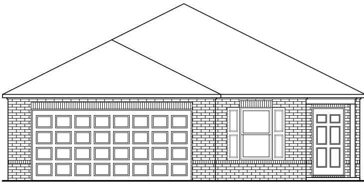
RC Bridgeport Elevation C
