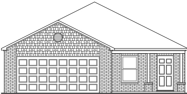
RC Armstrong II Elevation E
