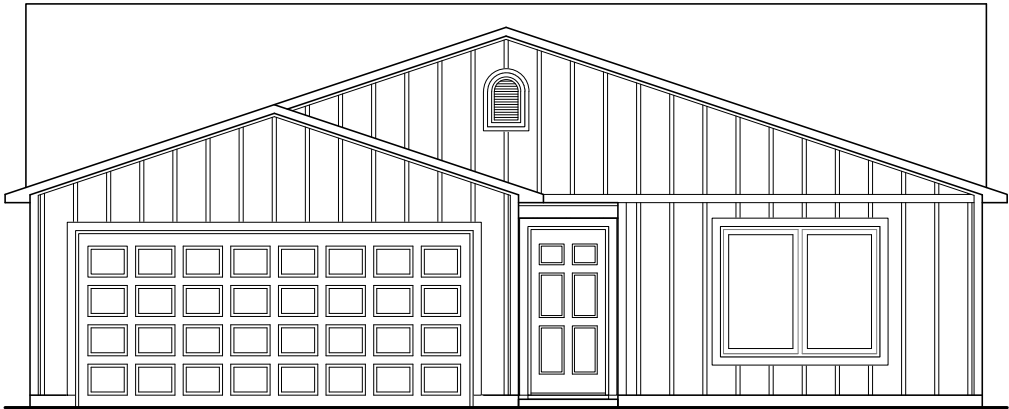
RC Palisade Elevation L
